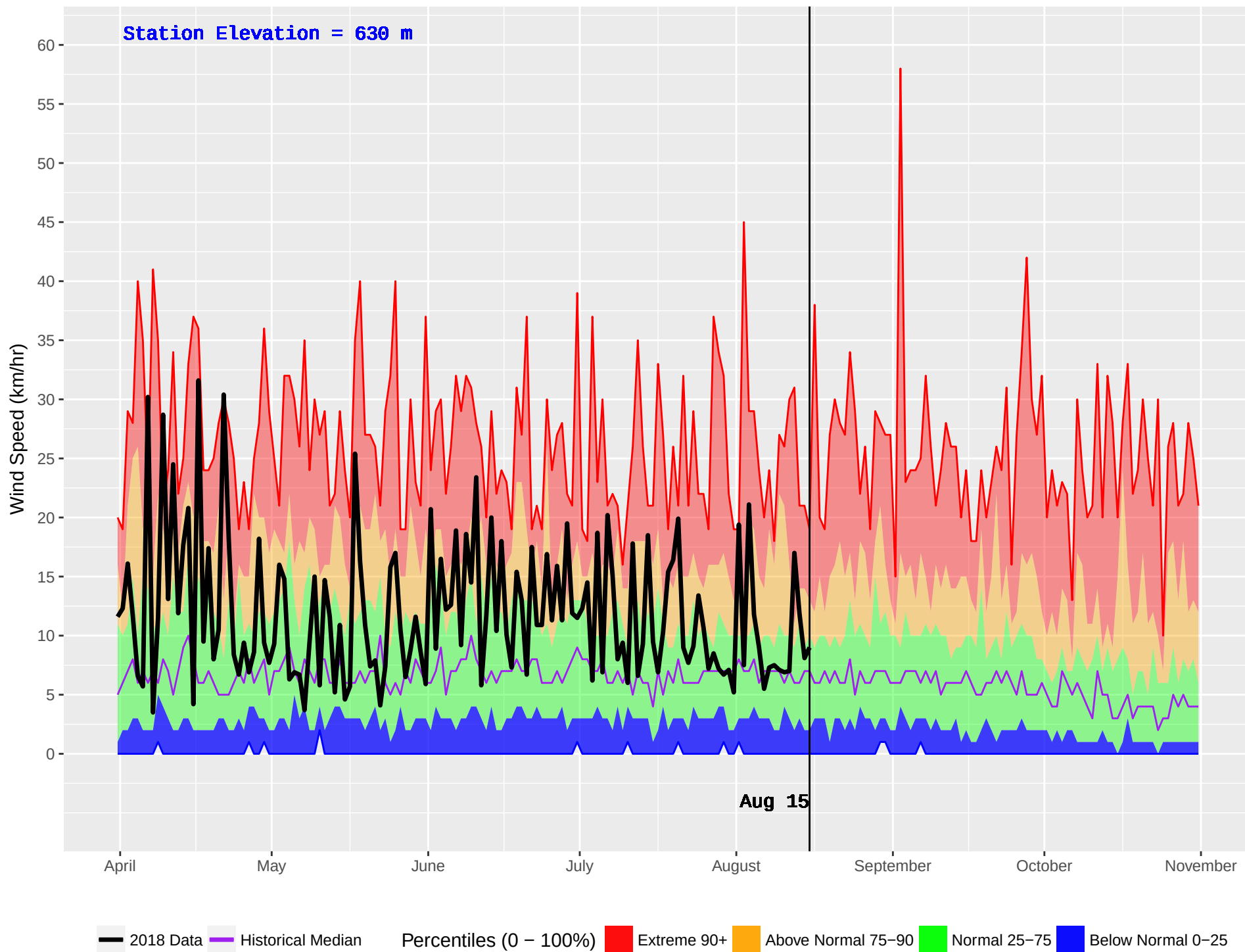
GRAND FORKS (392) : Historical (1981–2016) and Current (2018) Daily Wind Speed
