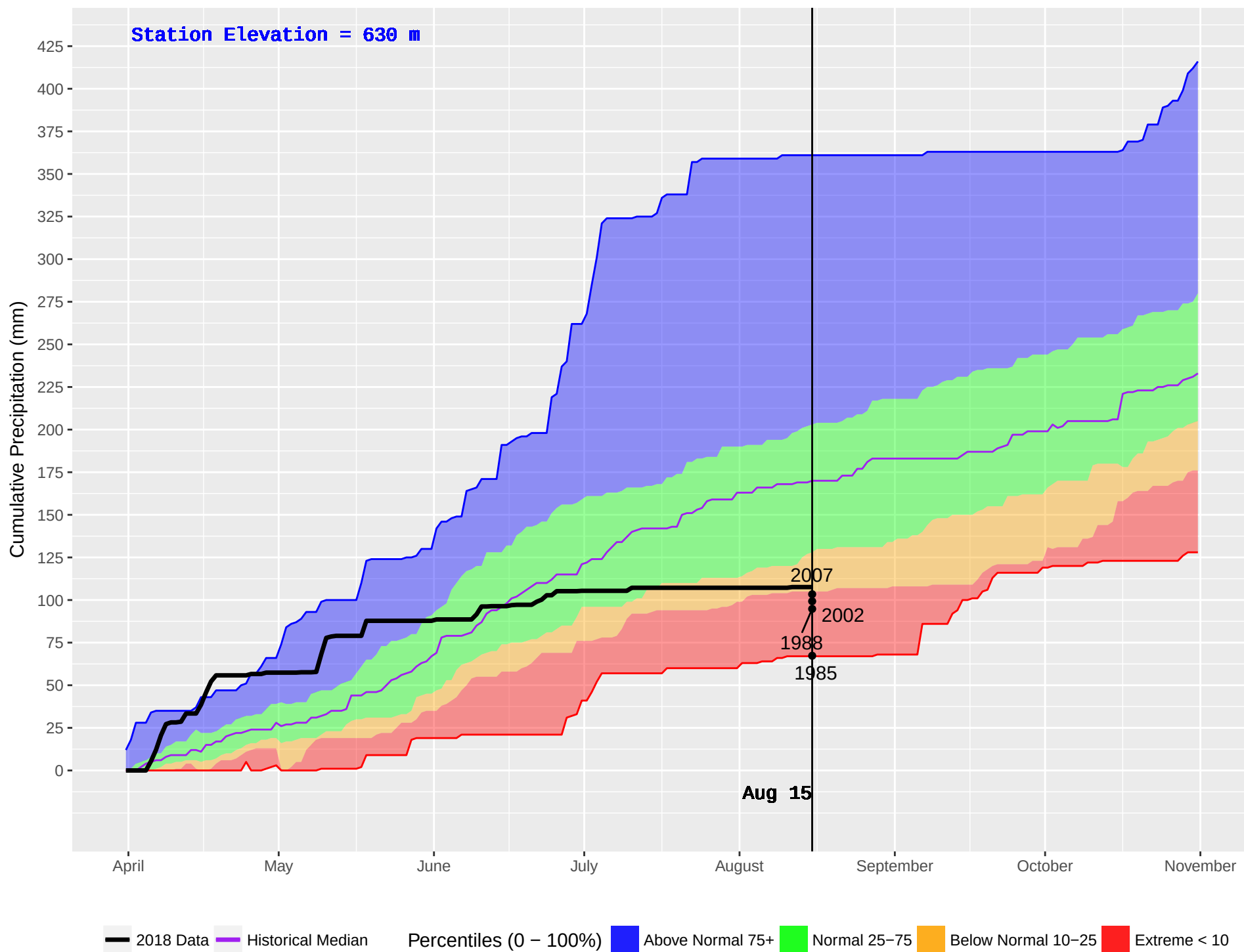
GRAND FORKS (392) : Historical (1981–2016) and Current (2018) Daily Cumulative Precipitation
